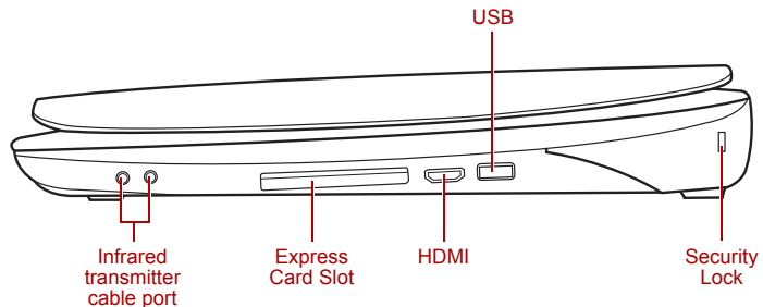
Figure 2-3 The right side of the computer
